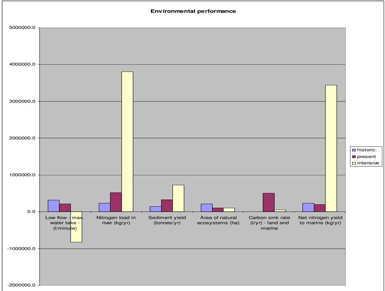
Figure 2: Environmental measures of Motueka catchment scenarios
